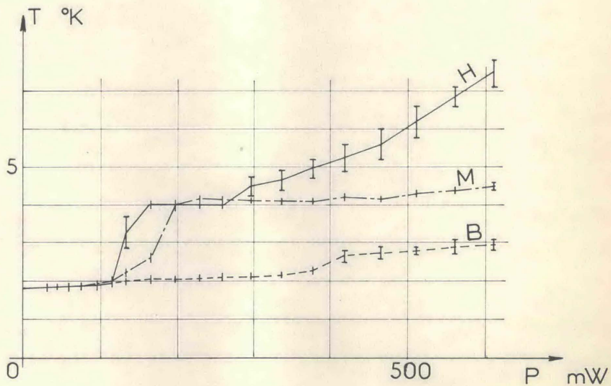
FIG.10 : Superfluid helium T = 1.8 K ; p = 1 atm
